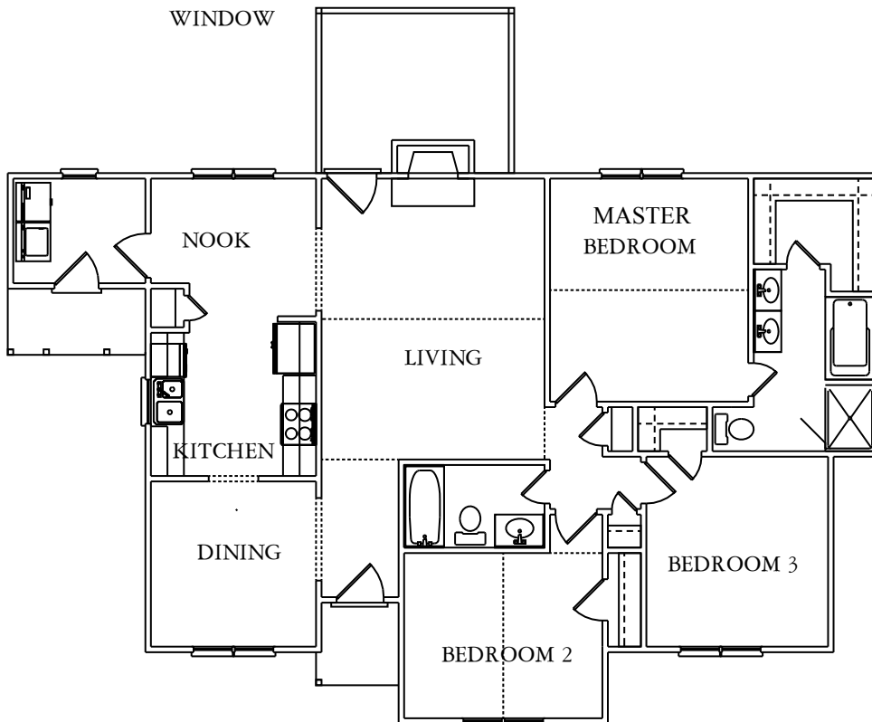
FLOOR PLAN
